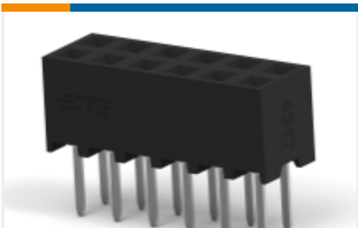
TE Part #1-2314812-2 12P,2MM,B-B,REC,DRV,2.0,0.1AU,TB, W/CAP
