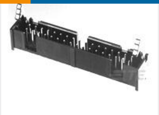
TE Part #1-1761608-3 IDC LOW PRO HDR 40P VERT SHT L
