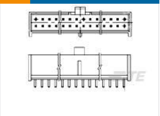
TE Part #1-1658549-6 FPH-2022T=FLXPAC HDR P 20 ST LF
