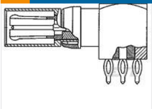
TE Part #148386-1 TYPE C,PIN ASSY.RTANG, RF
