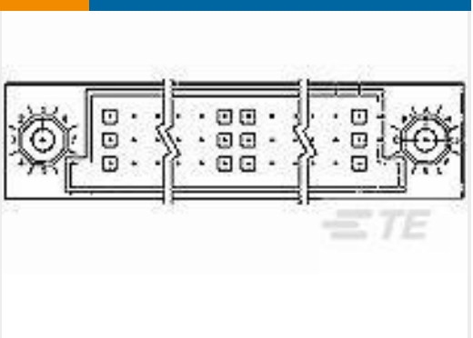
TE Part #1-5532433-1 ASSY,PIN,VERTICAL,HDI,LEAD-FRE
