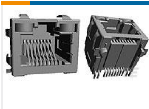
TE Part #6339191-4 MJ,RJ45,SMT,SHLD,LED (G/Y)
