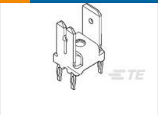
TE Part #216905-1 POSITIVE LOCK POWER RECEPTACLE TPPHBRZ
