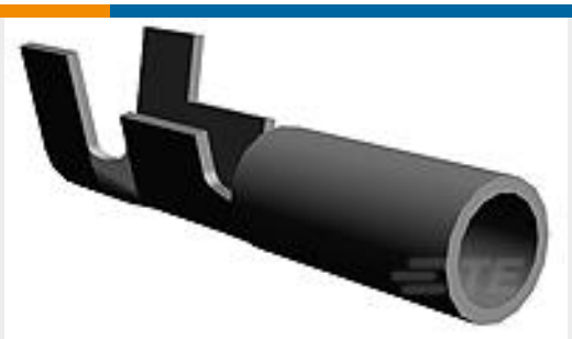
TE Part #1742350-1 PIN 2.08 DIA 22-18AWG TPBR
