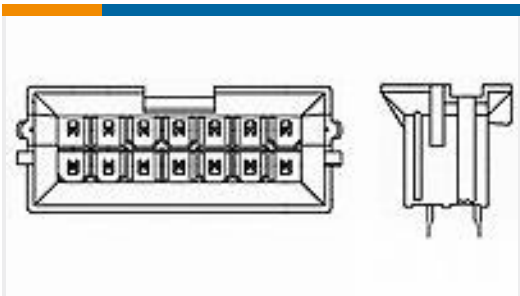
TE Part #1586588-4 4P VAL-U-LOK BMI VRT HDR V0
