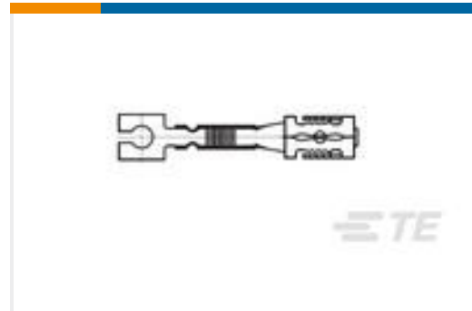
TE Part #1494211-1 SIZE(2.8) AMPLIVAR FASTON RECP
