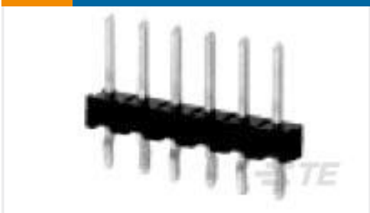
TE Part #104344-5 07 MODII HDR SRST B/A W/HD
