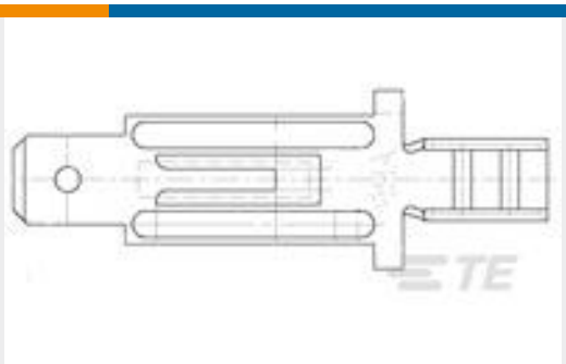
TE Part #1217006-1 250 FASTON,TAB,22-15 AWG,NPST
