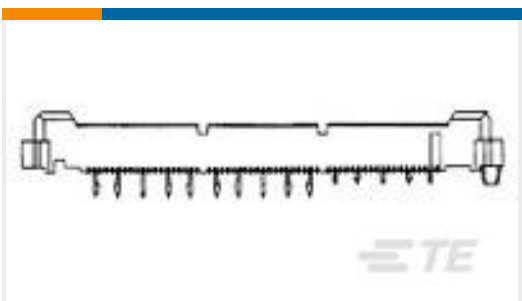
TE Part #5148116-5 ASSY,PIN,EUROCARD,TYPE C,LEAD-FREE,9% PO
