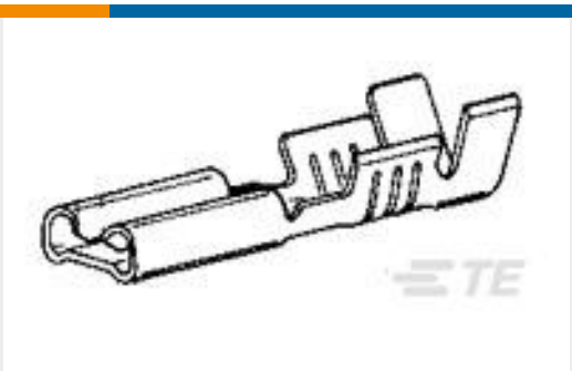
TE Part #140717-2 110 FASTON,REC.,22-18 AWG,PTBR
