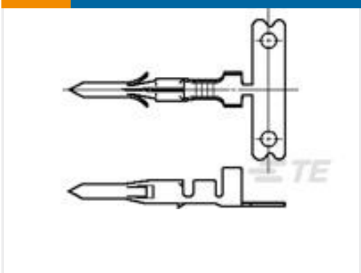
TE Part #794017-1 .062 CP&S PIN PTPBR L/P 24-18
