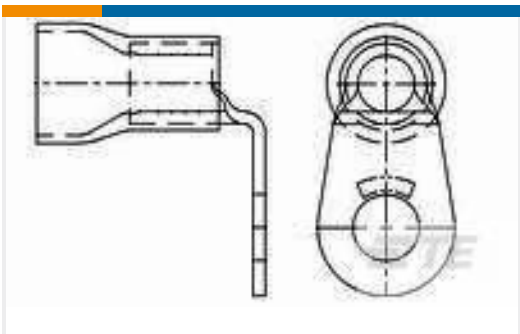
TE Part #1958413-1 TERMINAL R PG 4 AWG, 5/16, BENT 90
