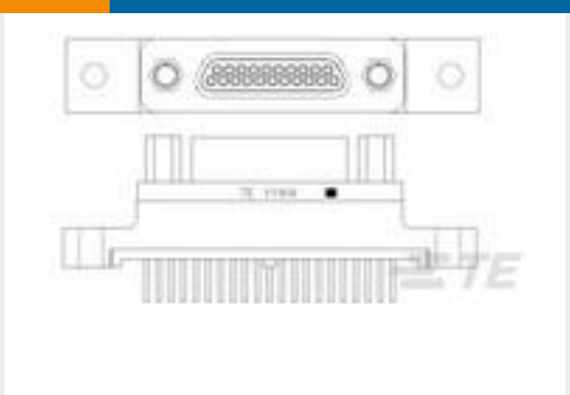
TE Part #1532268-3 M83513/22-C01NN = MCKS-N1-B-21PST1
