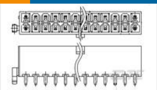
TE Part #1775099-8 ATX PWR CONN 1 BDLK 12 POS
