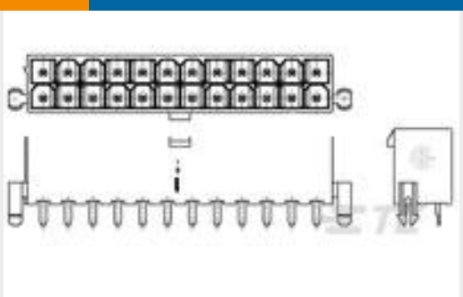
TE Part #2-1586040-4 24P VAL-U-LOK VRT HDR W/P V0
