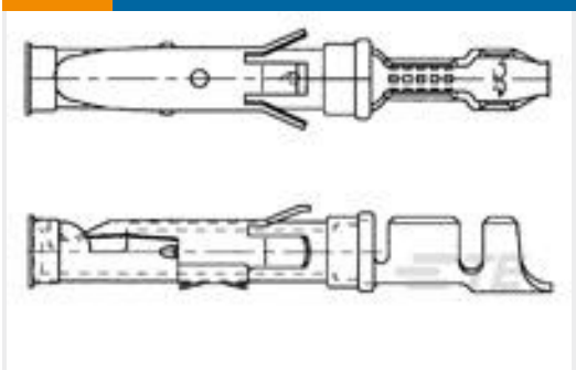
TE Part #163083-8 .062 DIA SOC.ASS.3+
