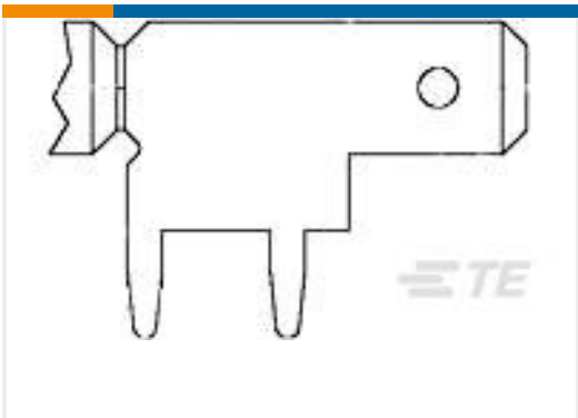
TE Part #1217062-1 187 FASTON,FLAG,PCB TAB,TNBR
