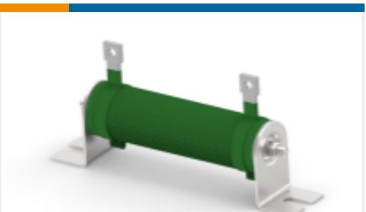
TE Part #1879455-2 Wirewound Resistor: Mineral, 2.5 Kw
