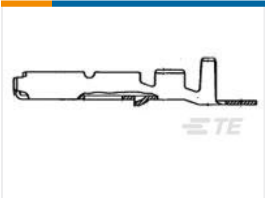
TE Part #172776-4 MIC MK-2 REC CONTACT LP
