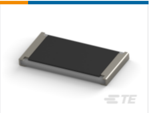
TE Part #1-2176071-3 SMD Power Resistor: 2 Watt, 3521 Series
