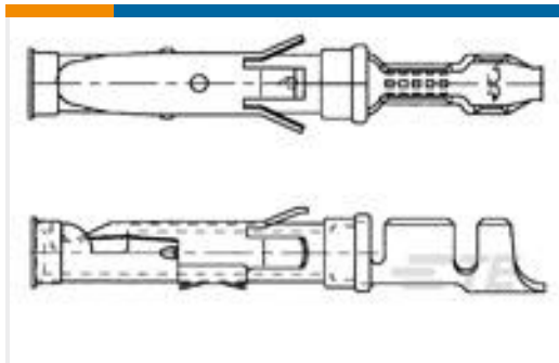
TE Part #163091-9 062 SOC.ASS. TYP3+
