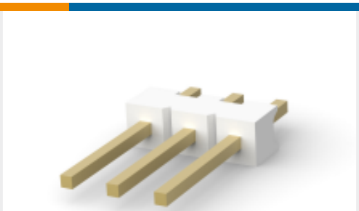
TE Part #5-644456-0 Polyester Vertical PCB Header: 2.54 mm, Breakaway, MTA 100
