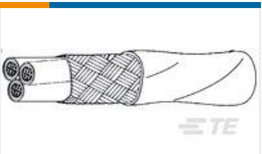
TE Part #7469813001 44A1131-24-3/93/9-3
