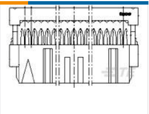
TE Part #1-215911-6 16 WAY GREY MK II RECP
