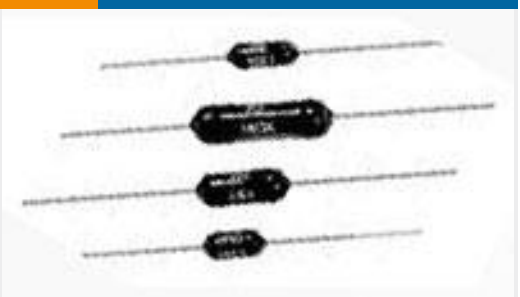
TE Part #9-1879672-4 H8 93R1 0.1% 25PPM
