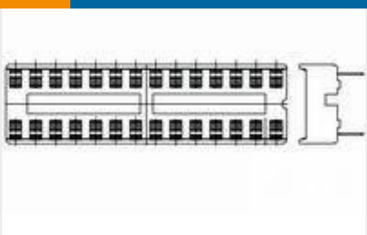
TE Part #1-2199298-8 24P,DIP SKT,300 CL,LDR,PB FREE
