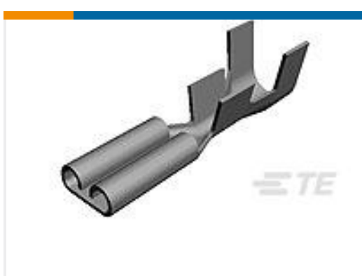
TE Part #140719-2 110 FASTON, REC., 22-18 AWG, TPBR
