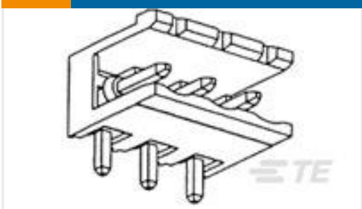
TE Part #282815-7 TERMI-BLOK HEADER,ASSY90 7P.5
