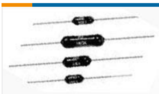
TE Part #3-1879666-9 H8 332K 0.1% 15PPM
