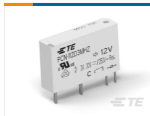
TE Part #1721081-7 PCN 3A/5A SLIM PCB RELAY 3VDC
