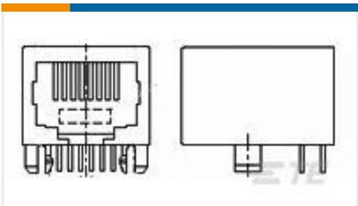
TE Part #1470648-1 RJ45,10P8C,LP,SIDE ENTRY,6u"
