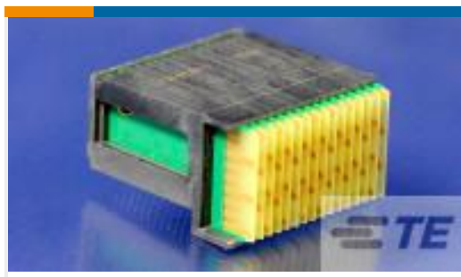
TE Part #1410139-2 MULTIGIG RT T2 .8 DC DF F-RGT
