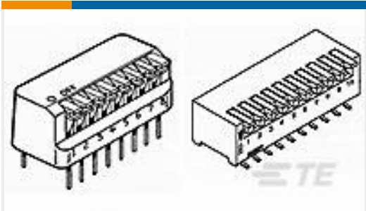
TE Part #1-5435802-7 RIGHT ANGLE DIP SW 6 P SEALED
