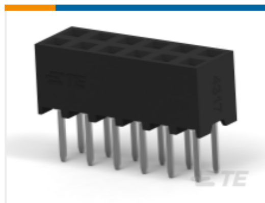
TE Part #1-2314820-2 12P, 2MM, B-B, REC, DRVT, 2.7, 0.1AU, TB
