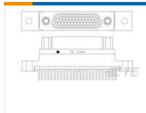
TE Part #1532277-2 M83513/25-D01CP = MCKS-C2-P-25SST1
