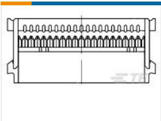
TE Part #1-1658526-6 609-2641LF FEM SOCKET, LEAD FREE
