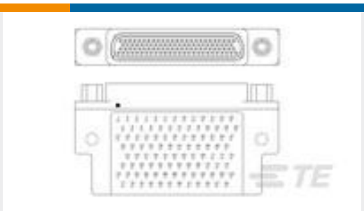
TE Part #1532265-1 M83513/15-H01CN = MCKS-C2-B-100SRT1
