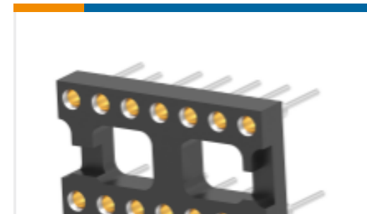
TE Part #1437539-5 DIP Socket: Standard, Stamped & Formed, Open, Gold
