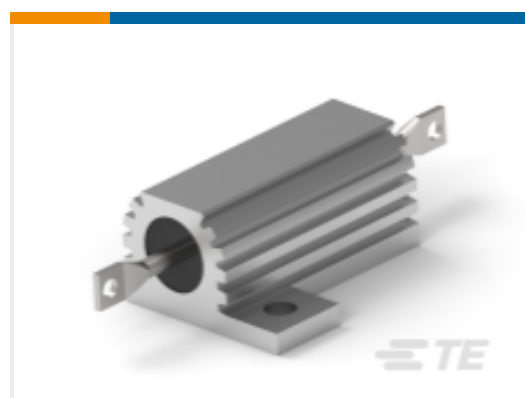
TE Part #1879071-6 Power Resistor: Aluminum Housed, 75 Watt
