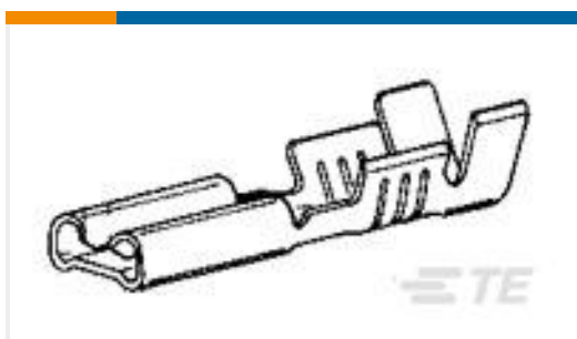
TE Part #160772-3 110 FASTON,REC.,26-22 AWG,TPBR
