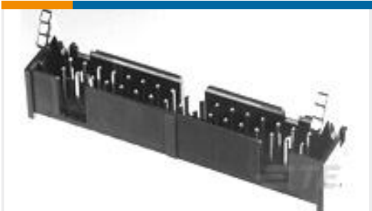
TE Part #1-1761606-3 IDC LOW PRO HDR 40P VERT LG LAT BLK
