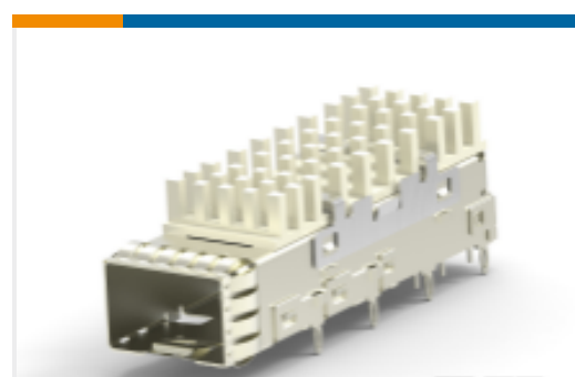
TE Part #2291634-2 SFP+ 1X1 CAGE ASSY, PF,WITH HEATSINK
