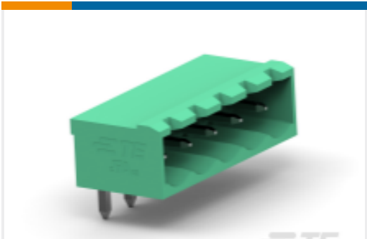
TE Part #1-2350513-5 15POS TB HDR 90 DEG, PITCH 5.0 &TL 4.5mm
