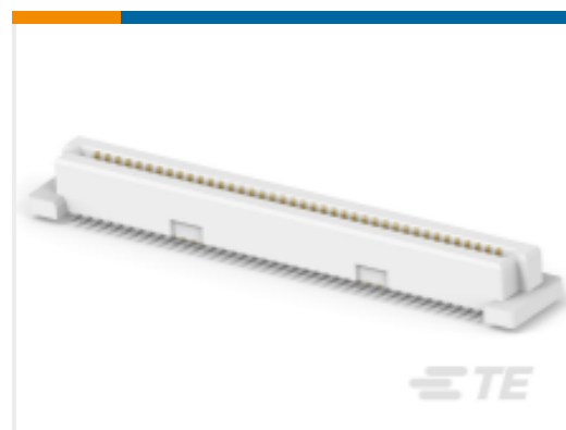
TE Part #1735481-3 Free Height Receptacle Conn: Board-Board, Vertical, 80, 0.8mm
