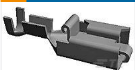
TE Part #170153-2 FF 250 TAB 18-14AWG PTBR LP
