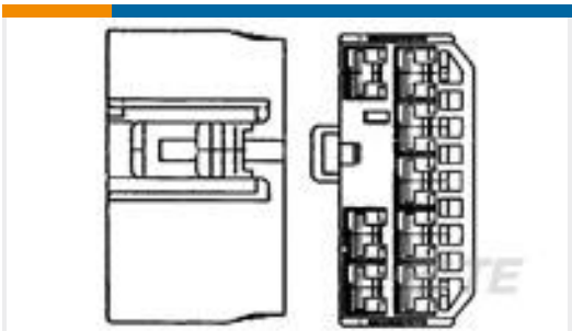
TE Part #175979-2 FF 187 PLUG HSG 8P NYLON BLACK
