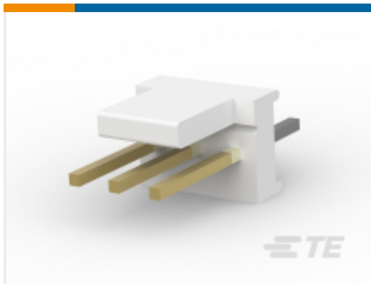
TE Part #3-641213-5 Polyester Vertical PCB Header: 2.54 mm, With Mating Alignment, Unshrouded
