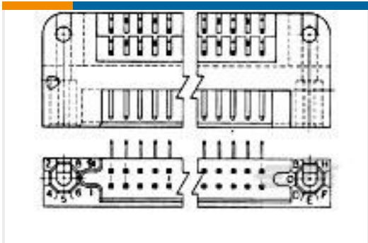
TE Part #1-531719-4 2 ROW BOX PIN 160 POS R/A
