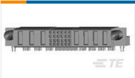
TE Part #1-6450170-8 MBXL R/A RCPT 4P+24S+3ACP
