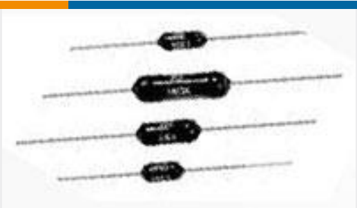
TE Part #1-1879628-5 H4P 510K 1% 100PPM
